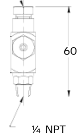
Injector FL 32 for direct mounting
