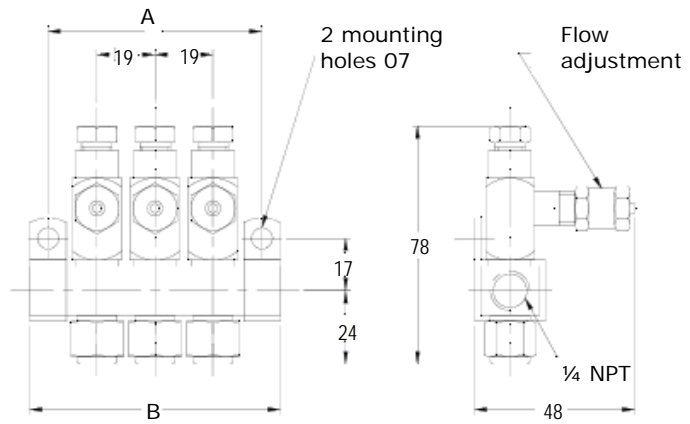
Injector FL 32 for manifold mounting
