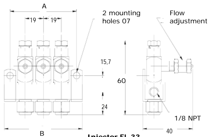
Injector FL 33 for manifold mounting
